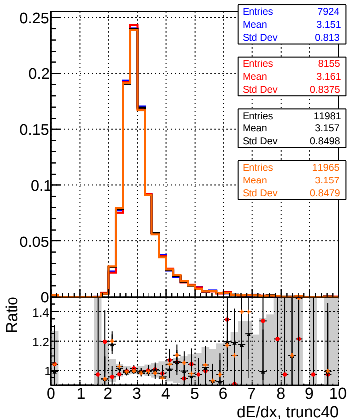
— DQM_original_step2_ttbar-phase1-newgeom — DQM_pixelCPETemplate_step2_ttbar-phase1-newgeom — DQM_pixelCPETemplateCutChiSquare5_step2_ttbar-phase1-newgeom — DQM_pixelCPETemplateCutChiSquare5Test_step2_ttbar-phase1-newgeom
