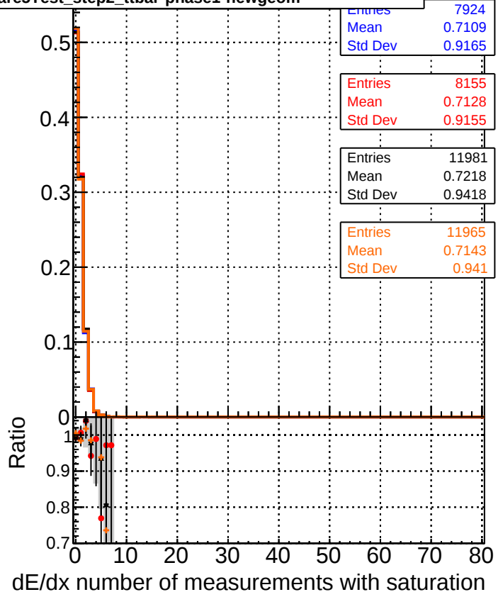
— DQM_original_step2_ttbar-phase1-newgeom — DQM_pixelCPETemplate_step2_ttbar-phase1-newgeom — DQM_pixelCPETemplateCutChiSquare5_step2_ttbar-phase1-newgeom — DQM_pixelCPETemplateCutChiSquare5Test_step2_ttbar-phase1-newgeom
