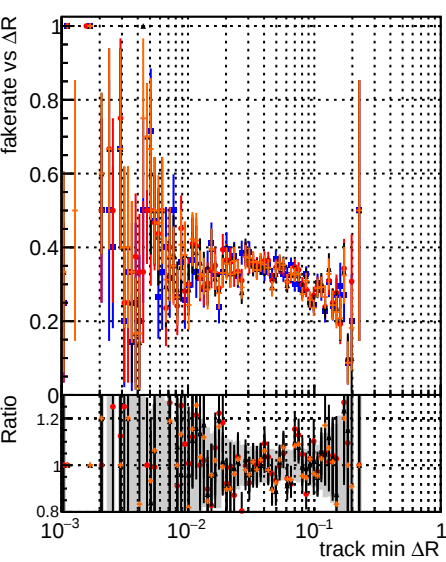
Fake rate vs \Delta R(\text{track, jet}) Legend: DOM original, step2, ttbar, phase1, newgeom pixelCPE, template, cutChisquare, test, step2, ttbar, phase1, newgeom pixelCPE, template, cutChisquare, test, step2, ttbar, phase1, newgeom
