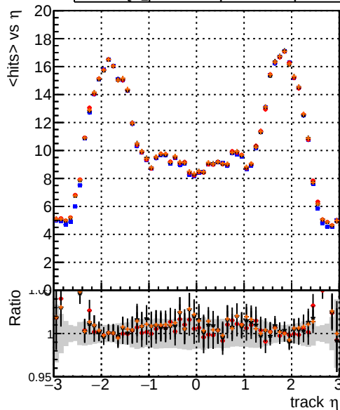
mean hits — DQM_original_step2_ttbar-phase1-newgeom — DQM_pixelCPETemplate_step2_ttbar-phase1-newgeom — DQM_pixelCPETemplateCutChiSquare5_test_step2_ttbar-phase1-newgeom — DQM_pixelCPETemplateCutChiSquare5Test_step2_ttbar-phase1-newgeom
