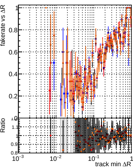
Fake rate vs \Delta R(\text{track, jet}) Legend: DOM original step2 ttbar-phase1 newgeom pixelCPE templateCuts chiSquare5 rest step2 ttbar-phase1 newgeom pixelCPE templateCuts chiSquare5
