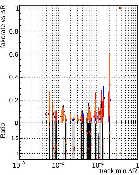
Fake rate vs ΔR(track, jet) Legend: DOM original_step2_ttbare-phase1-newgeom DOM pixelCPE-template_step2_ttbare-phase1-newgeom DOM pixelCPE-template_chiSquare5_test_step2_ttbare-phase1-newgeom DOM pixelCPE-template_chiSquare5_test_step2_ttbare-phase1-newgeom
