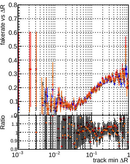
Fake rate vs \Delta R(\text{track, jet}) Legend: DOM original step2 ttbar-phase1-newgeom pixelCPE template cutchisquare 5test step2 ttbar-phase1-newgeom pixelCPE template cutchisquare 5test step2 ttbar-phase1-newgeom
