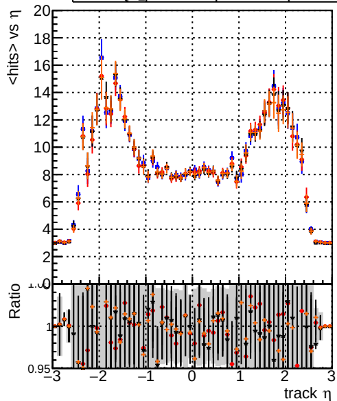
mean hits DQM_original_step2_ttbar-phase1-newgeom DQM_pixelCPETemplate_step2_ttbar-phase1-newgeom DQM_pixelCPETemplateCutChiSquare5_step2_ttbar-phase1-newgeom DQM_pixelCPETemplateCutChiSquare5Test_step2_ttbar-phase1-newgeom
