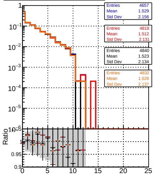
mean hits DQM_original_step2_ttbar-phase1-newgeom DQM_pixelCPETemplate_step2_ttbar-phase1-newgeom DQM_pixelCPETemplateCutChiSquare5_step2_ttbar-phase1-newgeom DQM_pixelCPETemplateCutChiSquare5Test_step2_ttbar-phase1-newgeom
