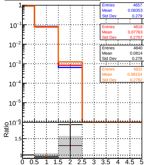
mean hits DQM_original_step2_ttbar-phase1-newgeom DQM_pixelCPETemplate_step2_ttbar-phase1-newgeom DQM_pixelCPETemplateCutChiSquare5_step2_ttbar-phase1-newgeom DQM_pixelCPETemplateCutChiSquare5Test_step2_ttbar-phase1-newgeom
