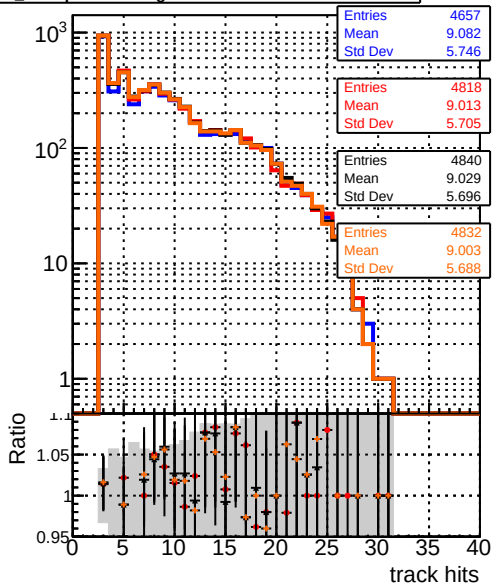
mean hits DQM_original_step2_ttbar-phase1-newgeom DQM_pixelCPETemplate_step2_ttbar-phase1-newgeom DQM_pixelCPETemplateCutChiSquare5_step2_ttbar-phase1-newgeom DQM_pixelCPETemplateCutChiSquare5Test_step2_ttbar-phase1-newgeom
