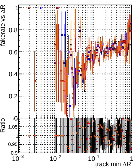
Fake rate vs \Delta R(\text{track, jet}) Legend: DOM original (blue squares) DOM step2 (red circles) DOM tbar-phase1 (black triangles) DOM newgeom (orange diamonds) pixelCPE (grey squares) TemplateCut (black circles) ChiSquare5 (grey squares) Square5 test (black circles)
