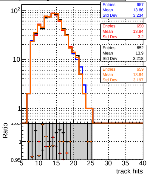
mean hit — DQM_original_step2_ttbar-phase1-newgeom — DQM_pixelCPETemplate_step2_ttbar-phase1-newgeom — DQM_pixelCPETemplateCutChiSquare5_step2_ttbar-phase1-newgeom — DQM_pixelCPETemplateCutChiSquare5Test_step2_ttbar-phase1-newgeom
