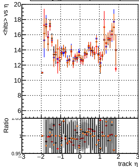
mean hit — DQM_original_step2_ttbar-phase1-newgeom — DQM_pixelCPETemplate_step2_ttbar-phase1-newgeom — DQM_pixelCPETemplateCutChiSquare5_step2_ttbar-phase1-newgeom — DQM_pixelCPETemplateCutChiSquare5Test_step2_ttbar-phase1-newgeom
