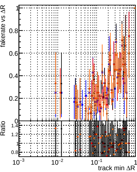
Fake rate vs \Delta R(\text{track, jet}) Legend: DOM original_step2_ttbare-phase1-newgeom DOM pixelCPE_Template_step2_ttbare-phase1-newgeom DOM pixelCPE_TemplateCutChiSquare5test_step2_ttbare-phase1-newgeom DOM pixelCPE_TemplateCutChiSquare5test_step2_ttbare-phase1-newgeom
