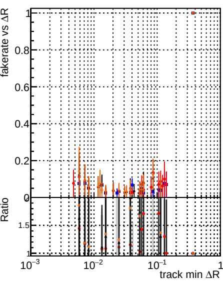
Fake rate vs \Delta R(\text{track, jet}) DOM original step2 ttbar-phase1 newgeom pixelCPE template cutChisquare 5test DOM pixelCPE template cutChisquare 5test step2 ttbar-phase1 newgeom
