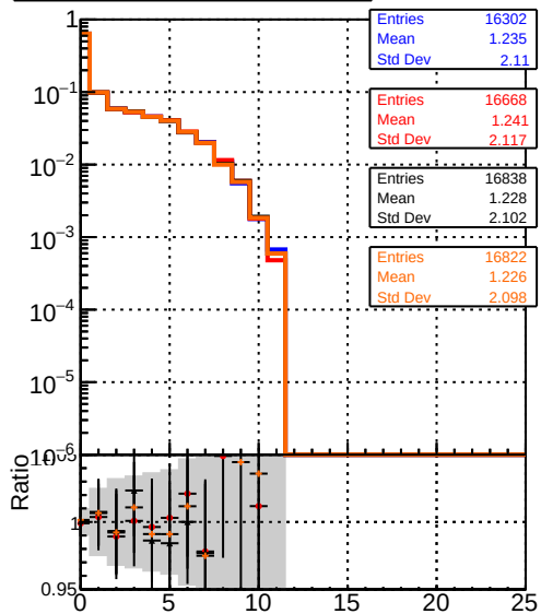
— DQM_original_step2_ttbar-phase1-newgeom — DQM_pixelCPETemplate_step2_ttbar-phase1-newgeom — DQM_pixelCPETemplateCutChiSquare5_step2_ttbar-phase1-newgeom — DQM_pixelCPETemplateCutChiSquare5Test_step2_ttbar-phase1-newgeom
