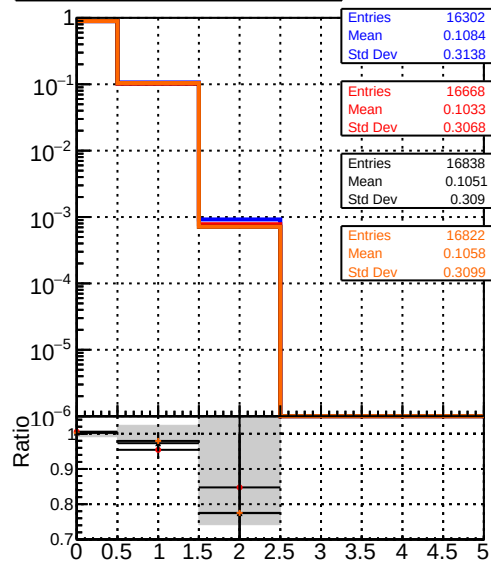
— DQM_original_step2_ttbar-phase1-newgeom — DQM_pixelCPETemplate_step2_ttbar-phase1-newgeom — DQM_pixelCPETemplateCutChiSquare5_step2_ttbar-phase1-newgeom — DQM_pixelCPETemplateCutChiSquare5Test_step2_ttbar-phase1-newgeom
