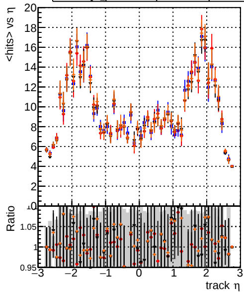
mean hit — DQM_original_step2_ttbar-phase1-newgeom — DQM_pixelCPETemplate_step2_ttbar-phase1-newgeom — DQM_pixelCPETemplateCutChiSquare5_step2_ttbar-phase1-newgeom — DQM_pixelCPETemplateCutChiSquare5Test_step2_ttbar-phase1-newgeom
