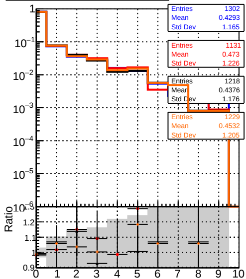
mean hit — DQM_original_step2_ttbar-phase1-newgeom — DQM_pixelCPETemplate_step2_ttbar-phase1-newgeom — DQM_pixelCPETemplateCutChiSquare5_step2_ttbar-phase1-newgeom — DQM_pixelCPETemplateCutChiSquare5Test_step2_ttbar-phase1-newgeom
