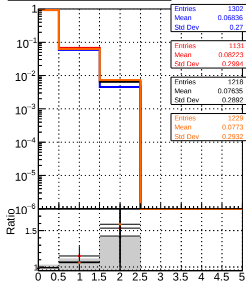
mean hit — DQM_original_step2_ttbar-phase1-newgeom — DQM_pixelCPETemplate_step2_ttbar-phase1-newgeom — DQM_pixelCPETemplateCutChiSquare5_step2_ttbar-phase1-newgeom — DQM_pixelCPETemplateCutChiSquare5Test_step2_ttbar-phase1-newgeom
