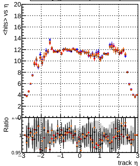
DQM_original_step2_ttbar-phase1-newgeom DQM_pixelCPETemplate_step2_ttbar-phase1-newgeom DQM_pixelCPETemplateCutChiSquare5_step2_ttbar-phase1-newgeom DQM_pixelCPETemplateCutChiSquare5Test_step2_ttbar-phase1-newgeom
