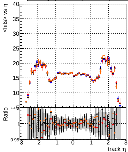
mean hits DQM_original_step2_ttbar-phase1-newgeom DQM_pixelCPETemplate_step2_ttbar-phase1-newgeom DQM_pixelCPETemplateCutChiSquare5_test_step2_ttbar-phase1-newgeom DQM_pixelCPETemplateCutChiSquare5Test_step2_ttbar-phase1-newgeom
