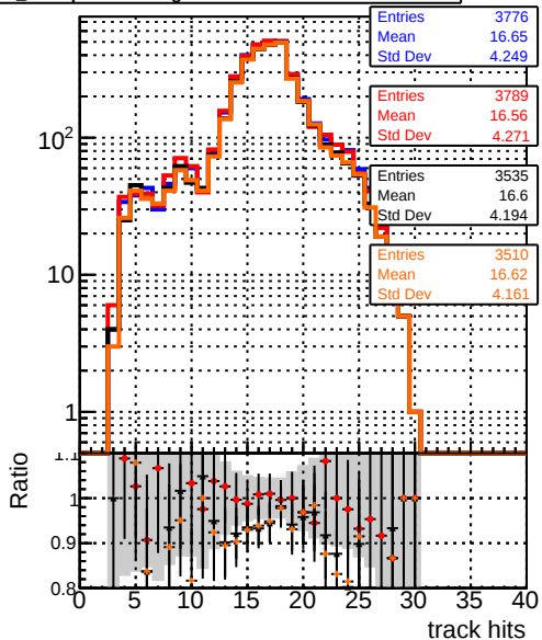
mean hits DQM_original_step2_ttbar-phase1-newgeom DQM_pixelCPETemplate_step2_ttbar-phase1-newgeom DQM_pixelCPETemplateCutChiSquare5_test_step2_ttbar-phase1-newgeom DQM_pixelCPETemplateCutChiSquare5Test_step2_ttbar-phase1-newgeom
