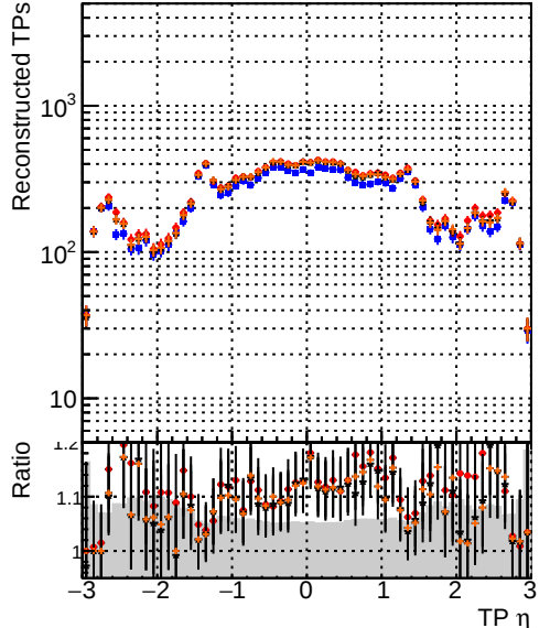
—•— DQM_original_step2_ttbar-phase1-newgeom —♦— DQM_pixelCPETemplate_step2_ttbar-phase1-newgeom —*— DQM_pixelCPETemplateCutChiSquare5_step2_ttbar-phase1-newgeom —+— DQM_pixelCPETemplateCutChiSquare5Test_step2_ttbar-phase1-newgeom
