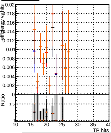
Efficiency vs hit Legend: DQM_original_step2_ttbbar-phase1-newgeom DQM_pixelCPETemplate_step2_ttbbar-phase1-newgeom DQM_pixelCPETemplateCutChiSquare5_step2_ttbbar-phase1-newgeom DQM_pixelCPETemplateCutChiSquare5Test_step2_ttbbar-phase1-newgeom
