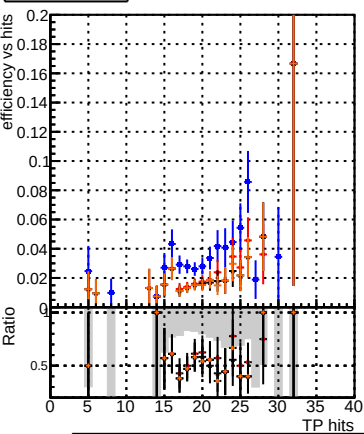
Efficiency vs hit Legend: DQM_original_step2_ttbar-phase1-newgeom DQM_pixelCPETemplate_step2_ttbar-phase1-newgeom DQM_pixelCPETemplateCutChiSquare5_step2_ttbar-phase1-newgeom DQM_pixelCPETemplateCutChiSquare5Test_step2_ttbar-phase1-newgeom
