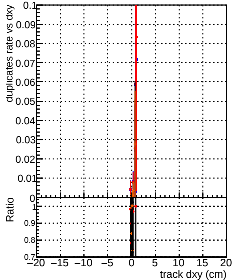
Square5_Test_step2 ttbar-phase1-newgeom
