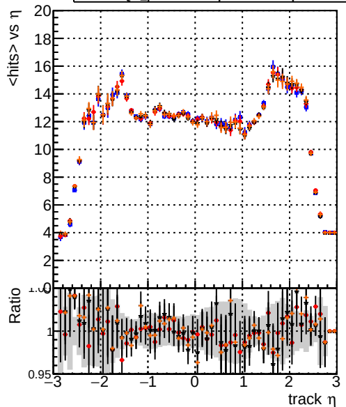
mean hits — DQM_original_step2_ttbbar-phase1-newgeom — DQM_pixelCPETemplate_step2_ttbbar-phase1-newgeom — DQM_pixelCPETemplateCutChiSquare5_step2_ttbbar-phase1-newgeom — DQM_pixelCPETemplateCutChiSquare5Test_step2_ttbbar-phase1-newgeom
