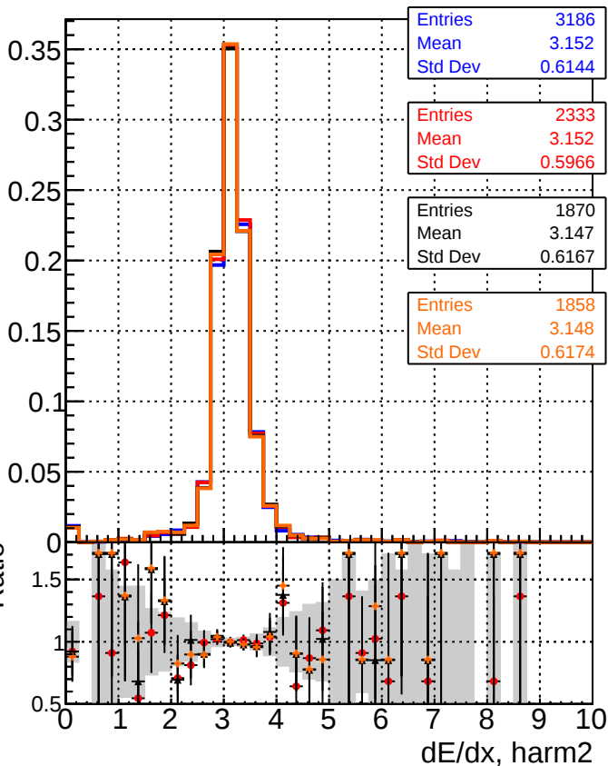
— DQM_original_step2_ttbar-phase1-newgeom — DQM_pixelCPETemplate_step2_ttbar-phase1-newgeom — DQM_pixelCPETemplateCutChiSquare5_step2_ttbar-phase1-newgeom — DQM_pixelCPETemplateCutChiSquare5Test_step2_ttbar-phase1-newgeom
