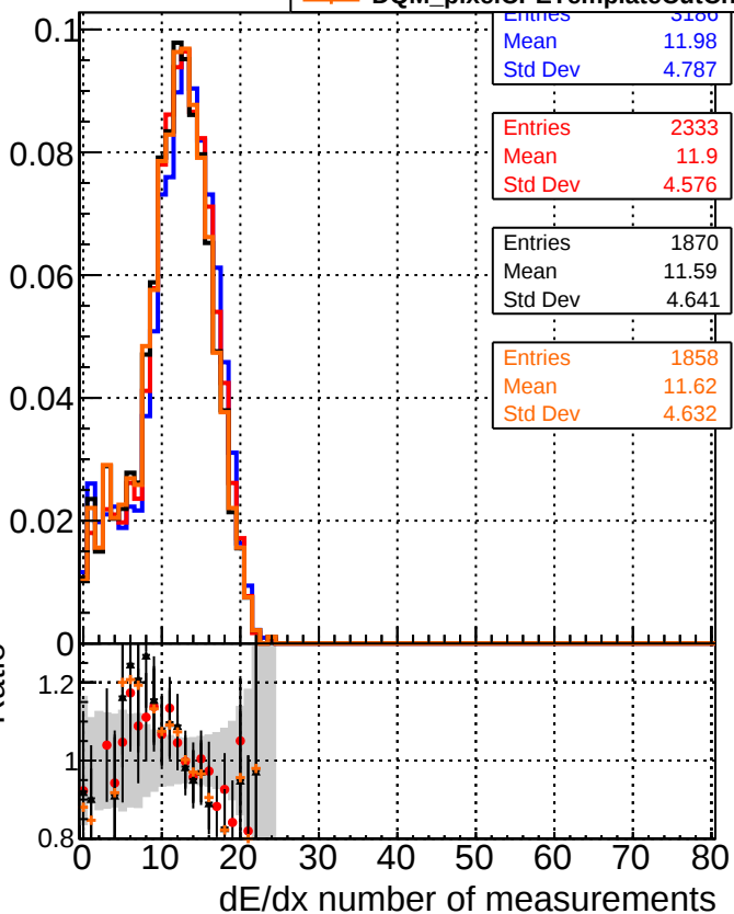
— DQM_original_step2_ttbar-phase1-newgeom — DQM_pixelCPETemplate_step2_ttbar-phase1-newgeom — DQM_pixelCPETemplateCutChiSquare5_step2_ttbar-phase1-newgeom — DQM_pixelCPETemplateCutChiSquare5Test_step2_ttbar-phase1-newgeom
