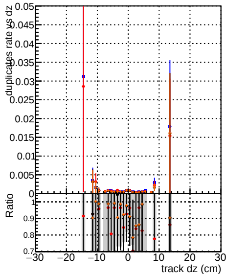
Square5_step2 ttbar-phase1-newgeom
