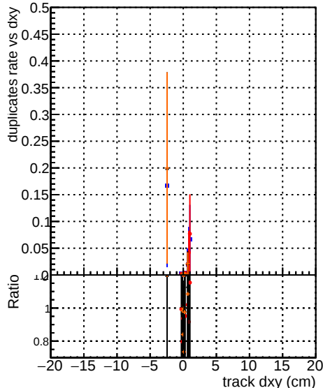
Square5_step2 ttbar-phase1-newgeom
