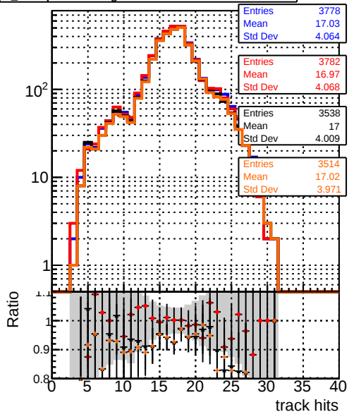
mean hits — DQM_original_step2_ttbar-phase1-newgeom — DQM_pixelCPETemplate_step2_ttbar-phase1-newgeom — DQM_pixelCPETemplateCutChiSquare5_test_step2_ttbar-phase1-newgeom — DQM_pixelCPETemplateCutChiSquare5Test_step2_ttbar-phase1-newgeom
