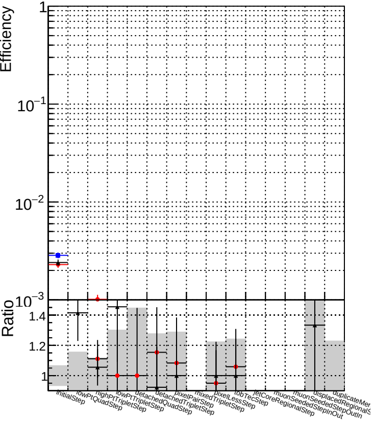
DQM_original_step2_ttbar-phase1-newgeom DQM_pixelCPETemplate_step2_ttbar-phase1-newgeom DQM_pixelCPETemplateCutChiSquare5_step2_ttbar-phase1-newgeom
