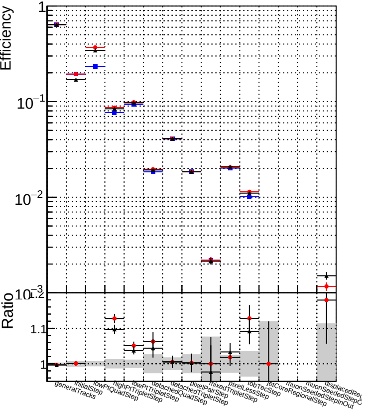
DQM_original_step2_ttbar-phase1-newgeom DQM_pixelICPETemplate_step2_ttbar-phase1-newgeom DQM_pixelICPETemplateCutChiSquare5_step2_ttbar-phase1-newgeom
