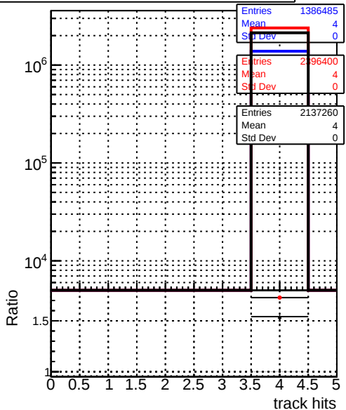
mean hits — DQM_original_step2_ttbar-phase1-newgeom — DQM_pixelCPETemplate_step2_ttbar-phase1-newgeom — DQM_pixelCPETemplateCutChiSquare5_step2_ttbar-phase1-newgeom
