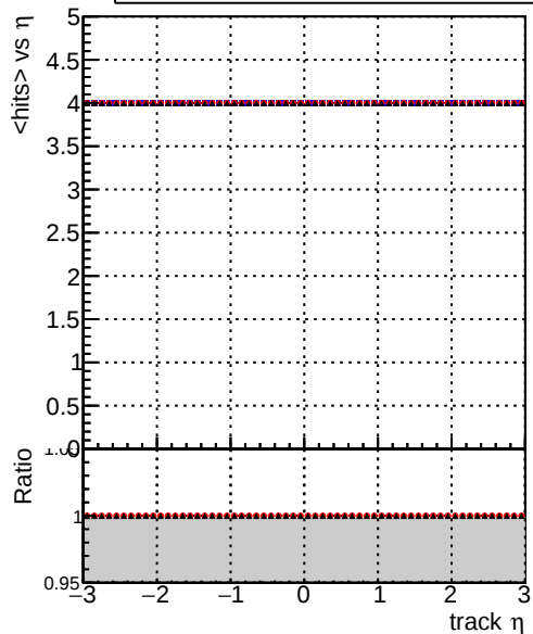
mean hits — DQM_original_step2_ttbar-phase1-newgeom — DQM_pixelCPETemplate_step2_ttbar-phase1-newgeom — DQM_pixelCPETemplateCutChiSquare5_step2_ttbar-phase1-newgeom
