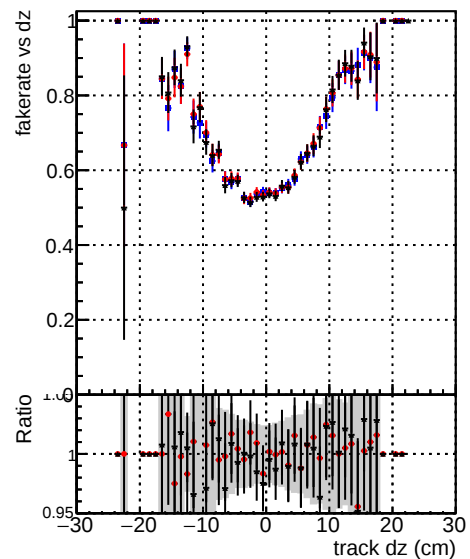
Fake rate vs dz Legend: DOM original_step2_tbar-phase1-newgeom pixelCPEtemplate_step2_tbar-phase1-newgeom DOM_pixelCPEtemplate_squares_step2_tbar-phase1-newgeom
