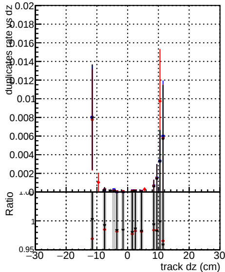
DOM original_step2_ttbarephase1-newgeom DOM pixelCPEtemplate_step2_ttbarephase1-newgeom DOM pixelCPEtemplatecurvesquares_step2_ttbarephase1-newgeom
