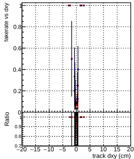
DOM original_step2_ttbarephase1-newgeom DOM pixelCPEtemplate_step2_ttbarephase1-newgeom DOM pixelCPEtemplatecurvesquares_step2_ttbarephase1-newgeom
