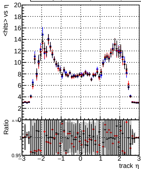
mean hits vs \eta — DQM_original_step2_ttbar-phase1-newgeom — DQM_pixelCPETemplate_step2_ttbar-phase1-newgeom — DQM_pixelCPETemplateCutChiSquare5_step2_ttbar-phase1-newgeom
