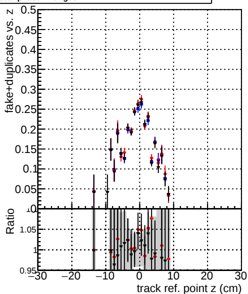
—●— DQM_original_step2_ttbbar-phase1-newgeom —●— DQM_pixelCPETemplate_step2_ttbbar-phase1-newgeom —●— DQM_pixelCPETemplateCutChiSquare5_step2_ttbbar-phase1-newgeom
