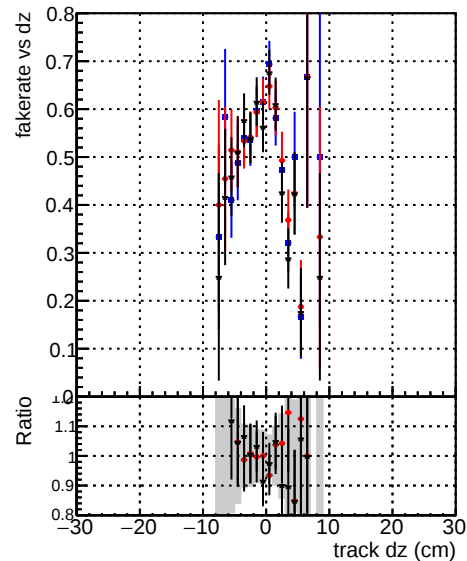
Fake rate vs dz Legend: DOM original_step2_ttbarenewgeom pixelCPEtemplate_step2_ttbarenewgeom DOM pixelCPEtemplatecurves_step2_ttbarenewgeom
