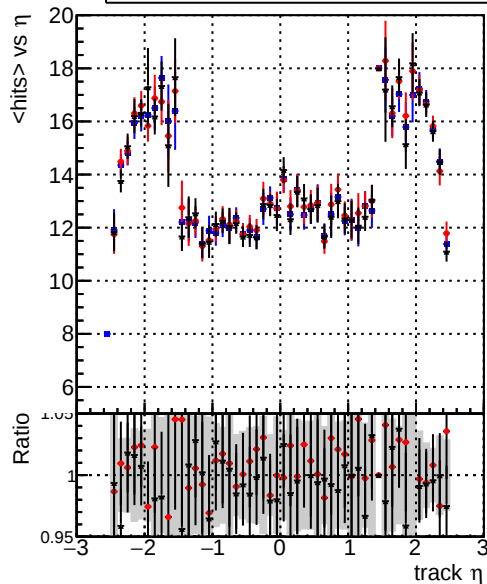
mean hit — DQM_original_step2_ttbar-phase1-newgeom — DQM_pixelCPETemplate_step2_ttbar-phase1-newgeom — DQM_pixelCPETemplateCutChiSquare5_step2_ttbar-phase1-newgeom
