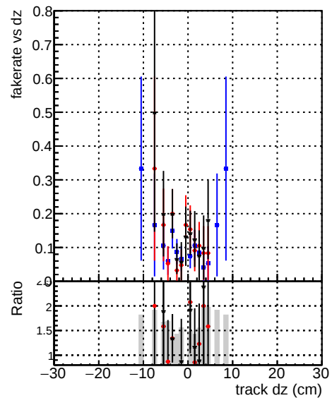
Fake rate vs dz Legend: DOM original_step2_ttbarenewgeom DOM pixelCPEtemplate_step2_ttbarenewgeom DOM pixelCPEtemplatecuttsquares_step2_ttbarenewgeom
