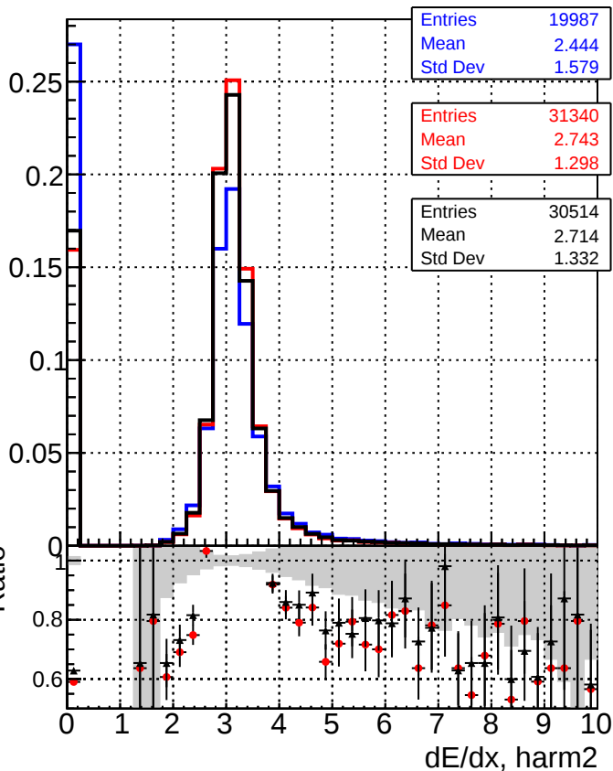
— DQM_original_step2_ttbar-phase1-newgeom — DQM_pixelCPETemplate_step2_ttbar-phase1-newgeom — DQM_pixelCPETemplateCutChiSquare5_step2_ttbar-phase1-newgeom
