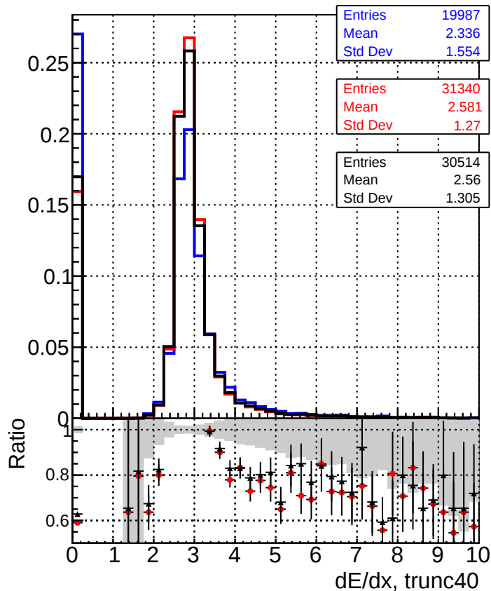
— DQM_original_step2_ttbar-phase1-newgeom — DQM_pixelCPETemplate_step2_ttbar-phase1-newgeom — DQM_pixelCPETemplateCutChiSquare5_step2_ttbar-phase1-newgeom
