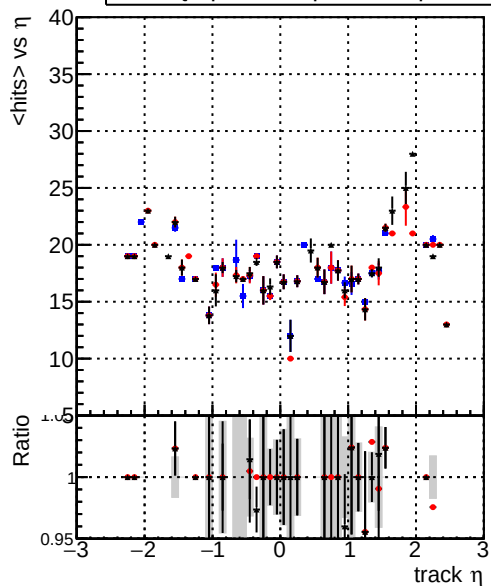
mean hit — DQM_original_step2_ttbar-phase1-newgeom — DQM_pixelCPETemplate_step2_ttbar-phase1-newgeom — DQM_pixelCPETemplateCutChiSquare5_step2_ttbar-phase1-newgeom
