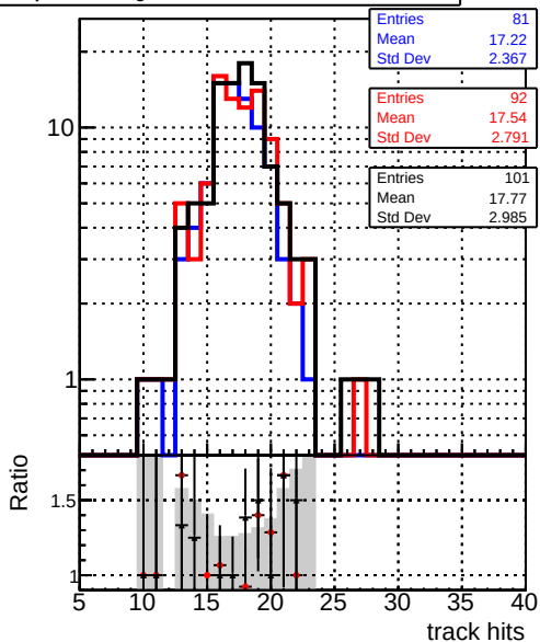
mean hit — DQM_original_step2_ttbar-phase1-newgeom — DQM_pixelCPETemplate_step2_ttbar-phase1-newgeom — DQM_pixelCPETemplateCutChiSquare5_step2_ttbar-phase1-newgeom
