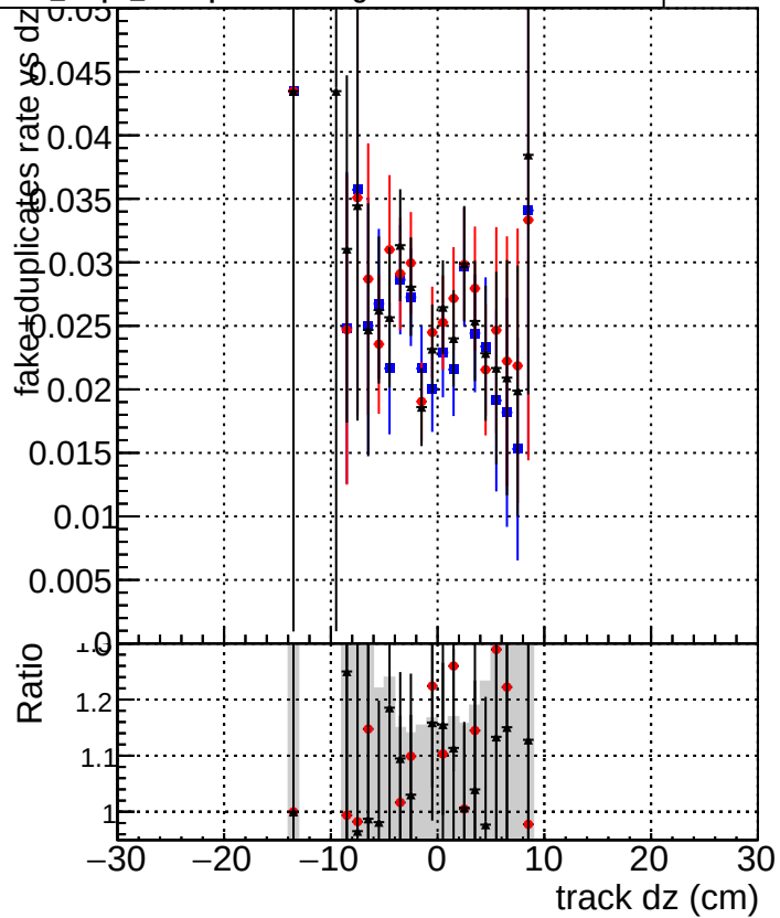
DQM_original_step2_ttbbar-phase1-newgeom DQM_pixelCPETemplate_step2_ttbbar-phase1-newgeom DQM_pixelCPETemplateCutChiSquare5_step2_ttbbar-phase1-newgeom
