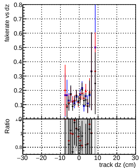
Fake rate vs dz Legend: DOM original_step2_ttbare1-newgeom DOM pixelCPEtemplate_step2_ttbare1-newgeom DOM pixelCPEtemplatecuttsquares_step2_ttbare1-newgeom
