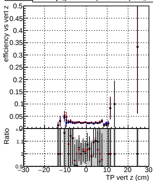
Efficiency vs. sim PV z —•— DQM_original_step2_ttbar-phase1-newgeom —•— DQM_pixelCPETemplate_step2_ttbar-phase1-newgeom —•— DQM_pixelCPETemplateCutChiSquare5_step2_ttbar-phase1-newgeom
