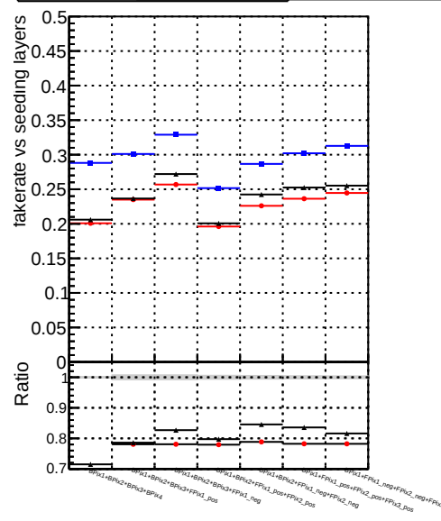
Fake rate vs. DOM original step2 tbar-phase1 newgeom DOM pixelCPE template cutchisquares step2 tbar-phase1 newgeom
