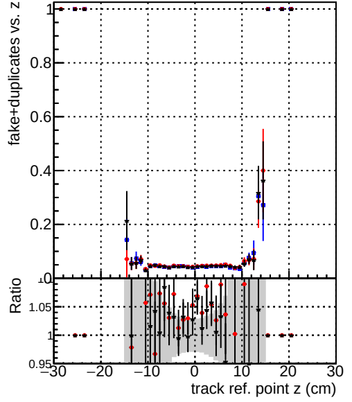
—●— DQM_original_step2_ttbar-phase1-newgeom —●— DQM_pixelCPETemplate_step2_ttbar-phase1-newgeom —●— DQM_pixelCPETemplateCutChiSquare5_step2_ttbar-phase1-newgeom
