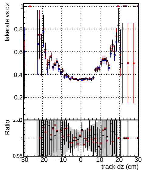
DOM original step2 ttbar-phase1-newgeom Fake rate vs d DOM pixelCPEtemplate step2 ttbar-phase1-newgeom DOM pixelCPEtemplateCutChiSquares step2 ttbar-phase1-newgeom
