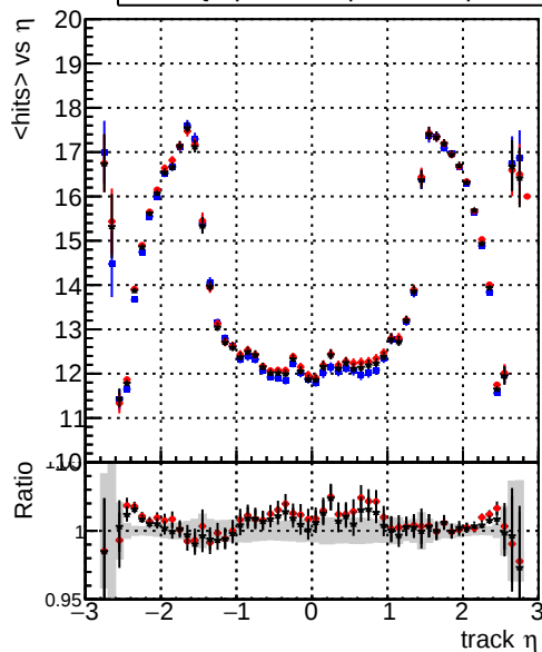
mean hits vs \eta — DQM_original_step2_ttbar-phase1-newgeom — DQM_pixelCPETemplate_step2_ttbar-phase1-newgeom — DQM_pixelCPETemplateCutChiSquare5_step2_ttbar-phase1-newgeom
