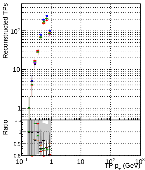
DOM pixel CPE Template Cut ChiSquare 10 step2 tbar phase1 newgeom N of sin DOM pixel CPE Template Cut ChiSquare 15 step2 tbar phase1 newgeom DOM pixel CPE Template Cut ChiSquare 20 step2 tbar phase1 newgeom DOM pixel CPE Template Cut ChiSquare 25 step2 tbar phase1 newgeom DOM pixel CPE Template Cut ChiSquare 30 step2 tbar phase1 newgeom DOM pixel CPE Template Cut ChiSquare 30 step2 tbar phase1 newgeom
