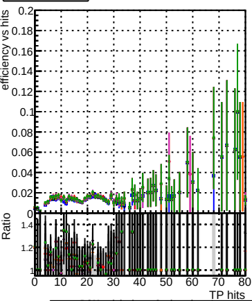
Efficiency vs hit DOM original_step2_ttbar-phase1-newgeom DOM pixelCPETemplate_step2_ttbar-phase1-newgeom DOM pixelCPETemplateCutChiSquare10_step2_ttbar-phase1-newgeom DOM pixelCPETemplateCutChiSquare15_step2_ttbar-phase1-newgeom DOM pixelCPETemplateCutChiSquare20_step2_ttbar-phase1-newgeom DOM pixelCPETemplateCutChiSquare30_step2_ttbar-phase1-newgeom
