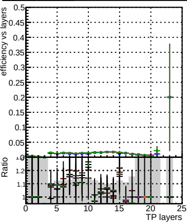
Efficiency vs hit DOM original_step2_ttbar-phase1-newgeom DOM pixelCPETemplate_step2_ttbar-phase1-newgeom DOM pixelCPETemplateCutChiSquare10_step2_ttbar-phase1-newgeom DOM pixelCPETemplateCutChiSquare15_step2_ttbar-phase1-newgeom DOM pixelCPETemplateCutChiSquare20_step2_ttbar-phase1-newgeom DOM pixelCPETemplateCutChiSquare30_step2_ttbar-phase1-newgeom
