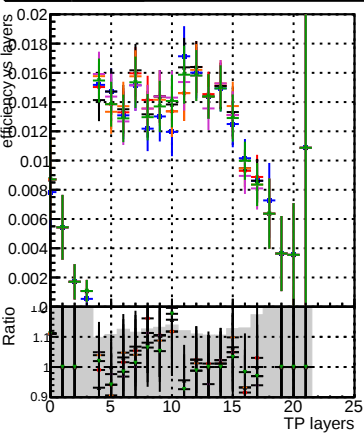
Efficiency vs hit Legend: DOM original_step2_ttbar-phase1-newgeom DOM pixelCPETemplate_step2_ttbar-phase1-newgeom DOM pixelCPETemplateCutChiSquare10_step2_ttbar-phase1-newgeom DOM pixelCPETemplateCutChiSquare15_step2_ttbar-phase1-newgeom DOM pixelCPETemplateCutChiSquare20_step2_ttbar-phase1-newgeom DOM pixelCPETemplateCutChiSquare30_step2_ttbar-phase1-newgeom
