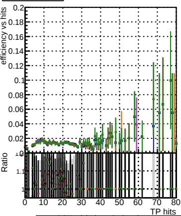
Efficiency vs hit Legend: DOM original_step2_ttbar-phase1-newgeom DOM pixelCPETemplate_step2_ttbar-phase1-newgeom DOM pixelCPETemplateCutChiSquare10_step2_ttbar-phase1-newgeom DOM pixelCPETemplateCutChiSquare15_step2_ttbar-phase1-newgeom DOM pixelCPETemplateCutChiSquare20_step2_ttbar-phase1-newgeom DOM pixelCPETemplateCutChiSquare30_step2_ttbar-phase1-newgeom
