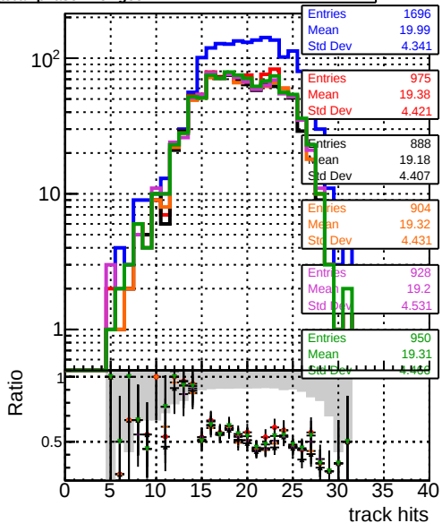
Legend: BOW, pixel, CDD, TemplateCut, ChiSquare, step2, tbar, phase1, newgeom mean hits
