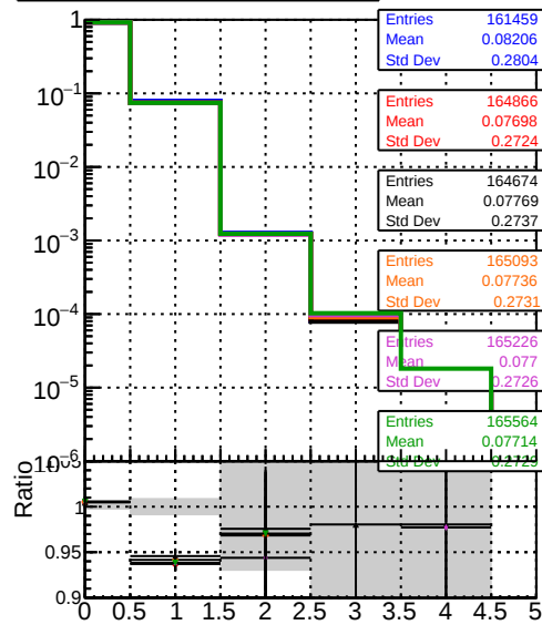
Legend: BDM original, BDM pixel, BDM pixel + template cut, BDM pixel + template cut + chi square, BDM pixel + template cut + chi square + step2 tbar phase1-newgeom, BDM pixel + template cut + chi square + step2 tbar phase1-newgeom, BDM pixel + template cut + chi square + step2 tbar phase1-newgeom, BDM pixel + template cut + chi square + step2 tbar phase1-newgeom
