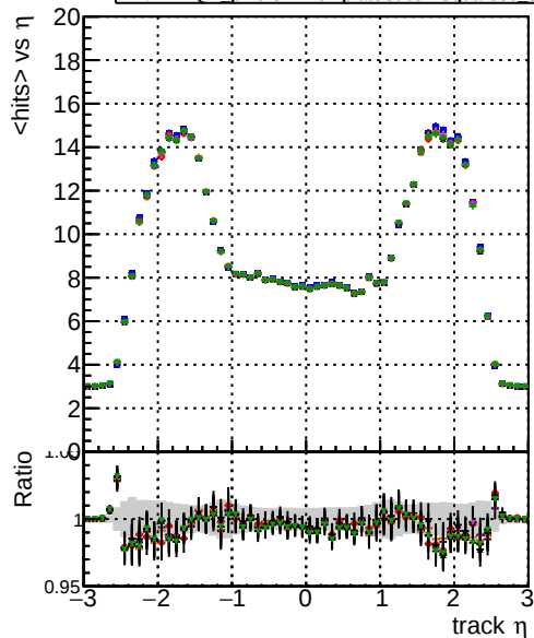
Legend: BDM original, BDM pixel, BDM pixel + template cut, BDM pixel + template cut + chi square, BDM pixel + template cut + chi square + step2 tbar phase1-newgeom, BDM pixel + template cut + chi square + step2 tbar phase1-newgeom, BDM pixel + template cut + chi square + step2 tbar phase1-newgeom, BDM pixel + template cut + chi square + step2 tbar phase1-newgeom
