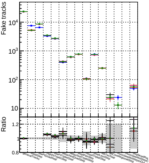
Number DOW pixe CCE ELE emb ate Cut Chi Square 15 step2 tibar phase1-newdecom DOW pixe CCE ELE emb ate Cut Chi Square 20 step2 tibar phase1-newdecom DOW pixe CCE ELE emb ate Cut Chi Square 20 step2 tibar phase1-newdecom
