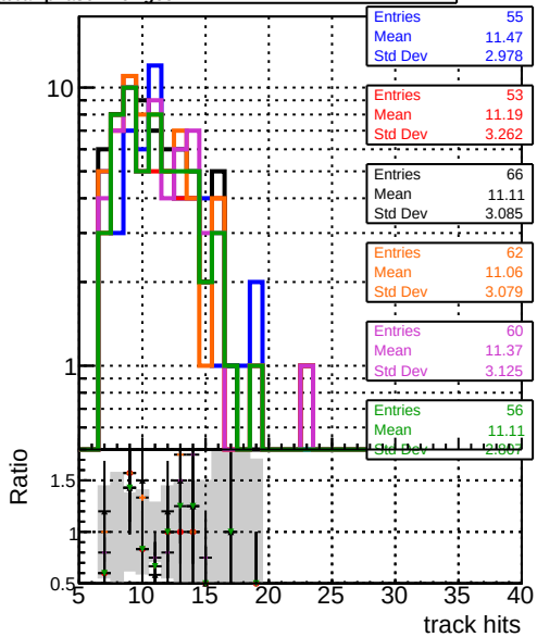
Legend: BDM, pixel, CDD, TemplateCut, ChiSquare, step2, tbar, phase1-newgeom mean hits
